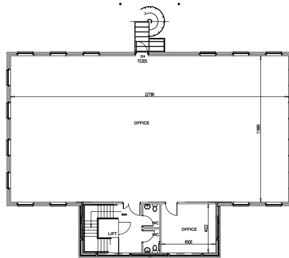
FIRST FLOOR LEVEL
