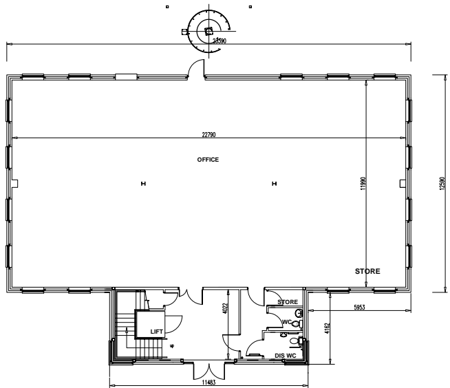
GROUND FLOOR LEVEL
