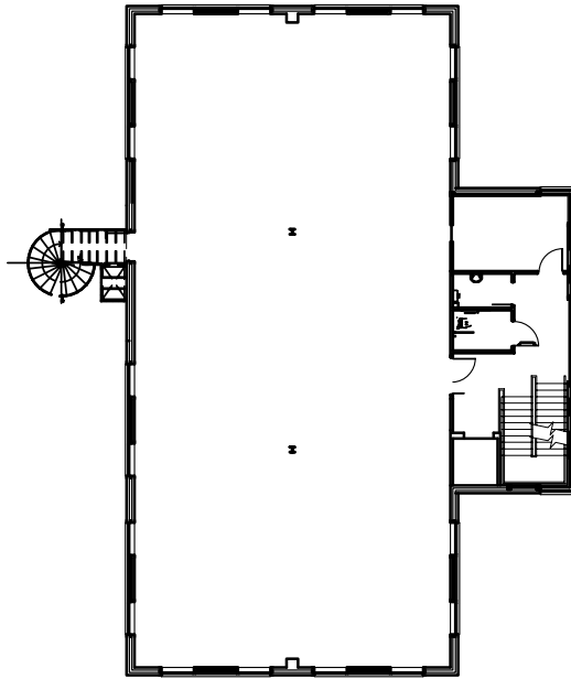
FIRST FLOOR LEVEL
