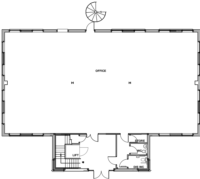
GROUND FLOOR LEVEL
